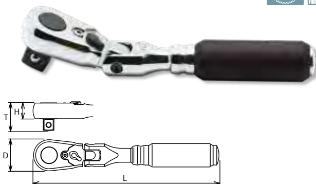
2726Z-3/8 Flexible Ratchet, Reversible (Short)
