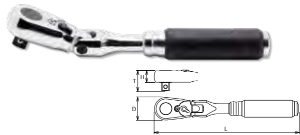
3726Z Flexible Ratchet, Reversible 3726Z-280
